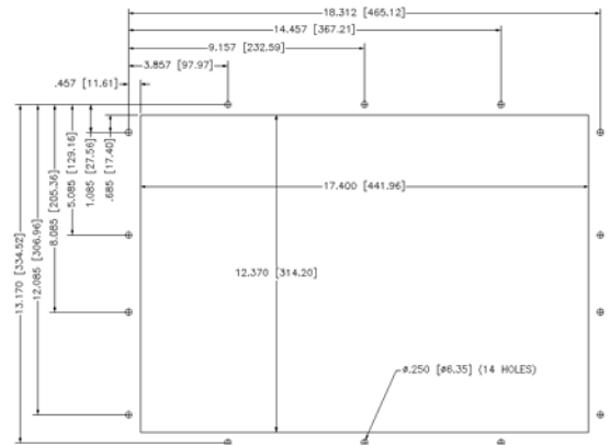
4615KPM(T) Cutout
