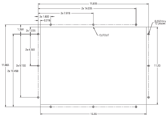
4615T Cutout
