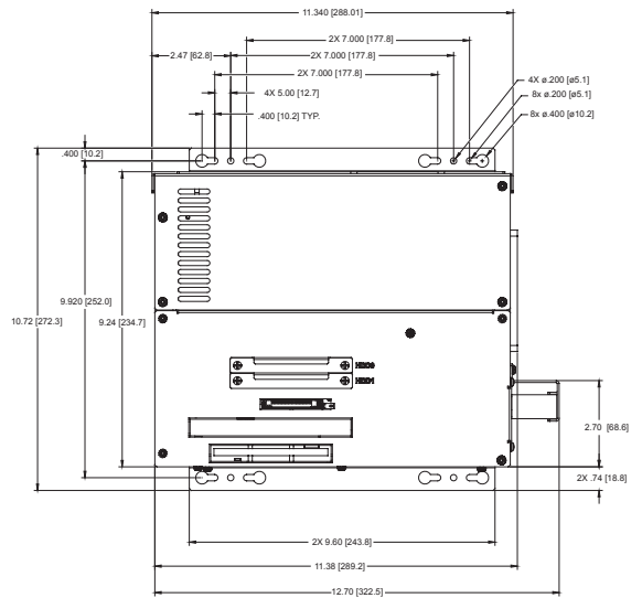
1546 Wall Mounting
