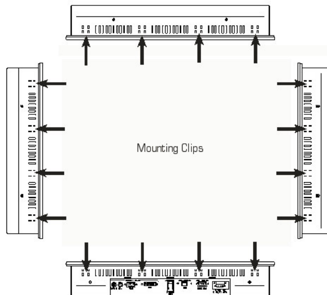
Figure 2-3. Mounting Clip Locations
